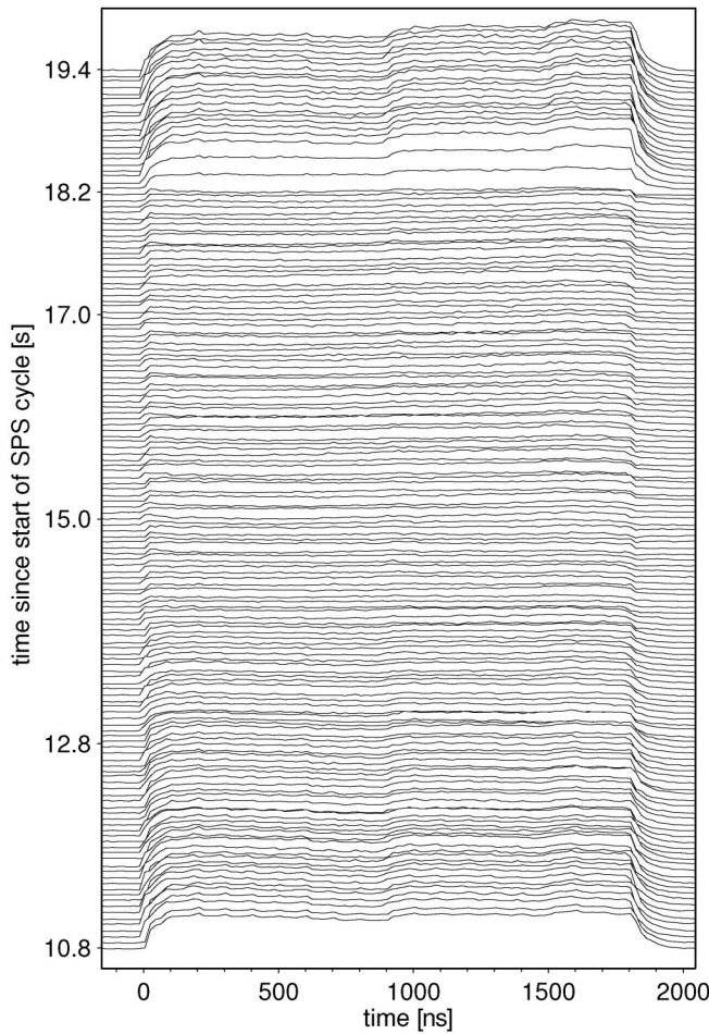
FIG. 9. Mountain range of phase pickup. The 800 MHz system is off and the rf AM is switched on at 12.8 s (64 GeV).
