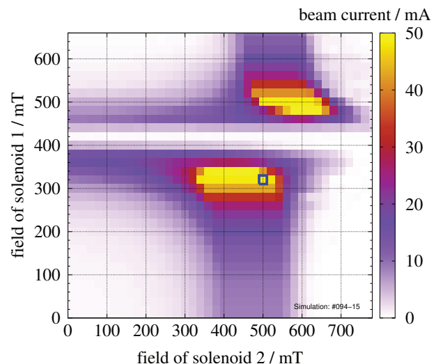
Figure 1: Transmission through the first LEBT section and the chopper system, evaluated at the exit of the chopper system. The best setting is highlighted with a blue square.
