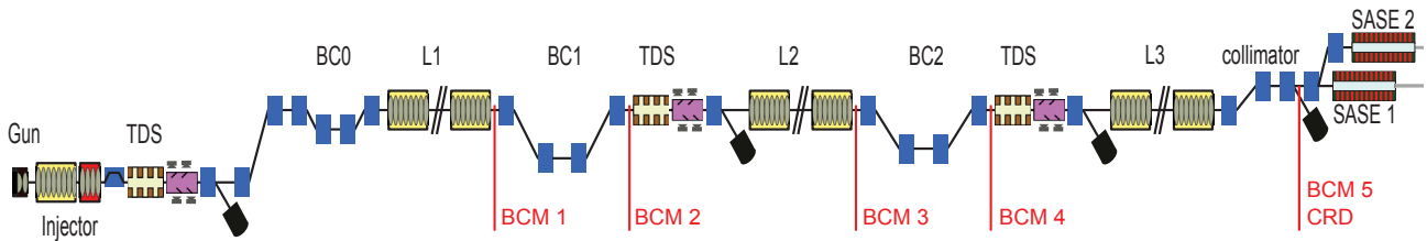
Figure 1: Main components of European XFEL.
