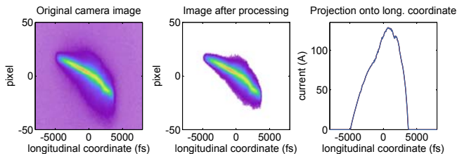
Figure 2: Example of data analysis. Image taken with ICCD camera in the straight section with LuAG screen. Left: original camera image. Middle: ROI of the image after processing. Right: longitudinal profile.
