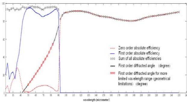
Figure 6. First and zero order efficiencies and first order diffracted angles for a RBG with 20 grooves/mm and blaze angle of 26.75° for S-polarization.
