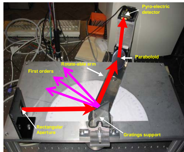
Figure 8. The mounting used for studies on distribution and efficiency of different orders at FELIX.
