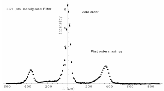
Figure 3: TG-Spectrometer is illuminated by CDR and a 357 \mu\text{m} band-pass filter is in the front of the detector.
