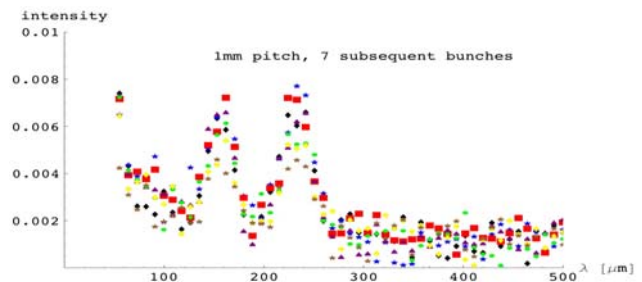
Figure 5. Bunch to bunch spectra made by TG spectrometer.
