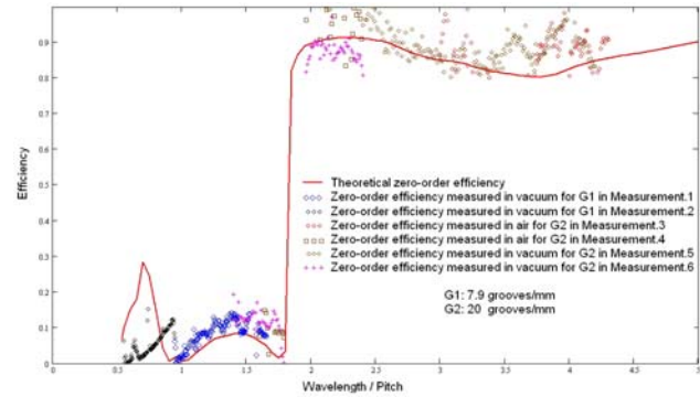
Figure 7. Theoretical zero-order (solid-red) and measured zero-order for two different gratings in air and vacuum.
