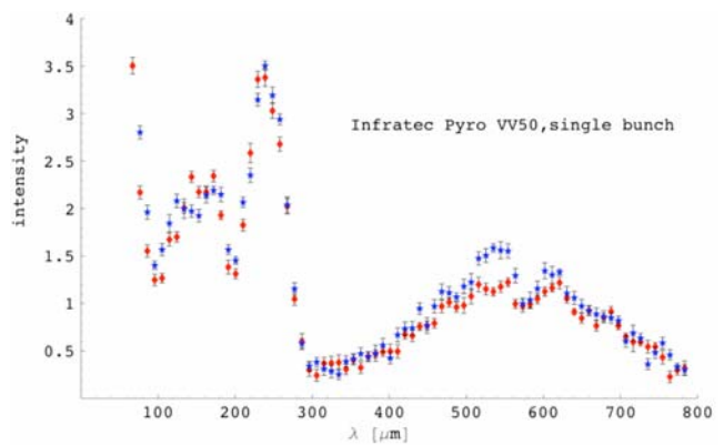
Figure 4. TG-Spectrometer is illuminated by CDR, no filters.
