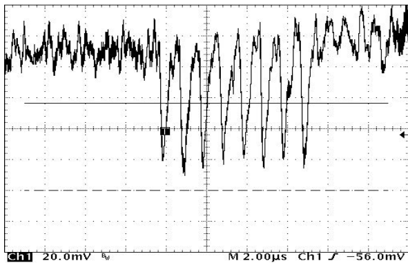
Figure 1: Signal from a Pyroelectric sensor for 8 subsequent bunches of InC charge in first spectroscopic order. The wavelength range covered by the detector is about 40 \mu\text{m} .
