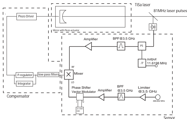
Figure 3: Schematic of the synchronisation unit.
