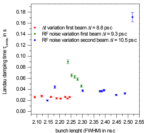
Figure 13: Landau damping time at 40 GeV. \Delta l is the average bunch lengthening per dipole kick for a measurement series.
