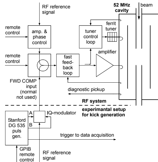
Figure 1: The 52 MHz RF System for an accelerating cavity and the intervention for the RF kick production.
